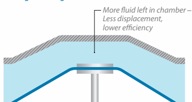
Conventional Diaphragm During Discharge Stroke
