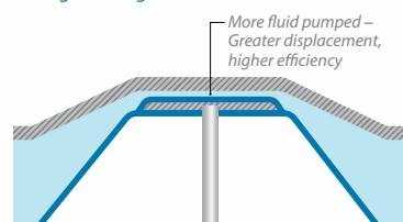
Full-Stroke PTFE Diaphragm During Discharge Stroke
