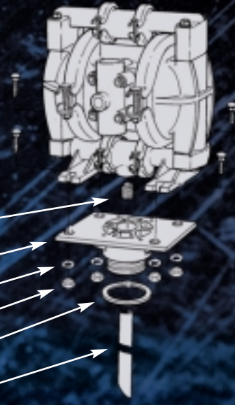
A1, P1 & T1 Installation
