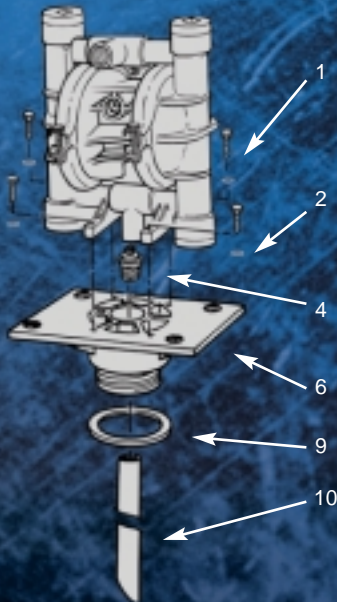
A.025 & P.025 Installation
