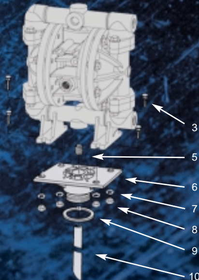
P100 Advanced™ Installation
